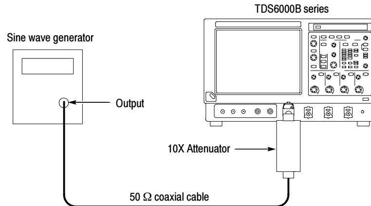
Figure 4-17: Initial test hookup
